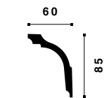
GL NOMASTYL® 85 x 60 x 2000 mm
