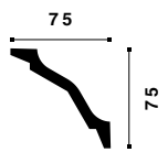
WT26 WALLSTYL® 75 x 75 x 2000mm
