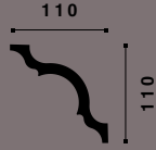
A NOMASTYL® 110 x 110 x 2000 mm
