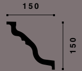
TL NOMASTYL® 150 x 150 x 2000 mm
