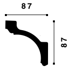
Z20 ARSTYL® 87 x 87 x 2000 mm
